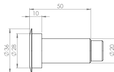
36MM FLAT STAINLESS STEEL SENSOR
