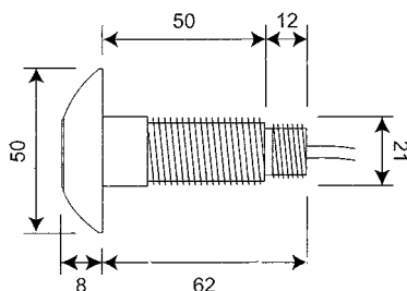
50MM STAINLESS STEEL SENSOR
