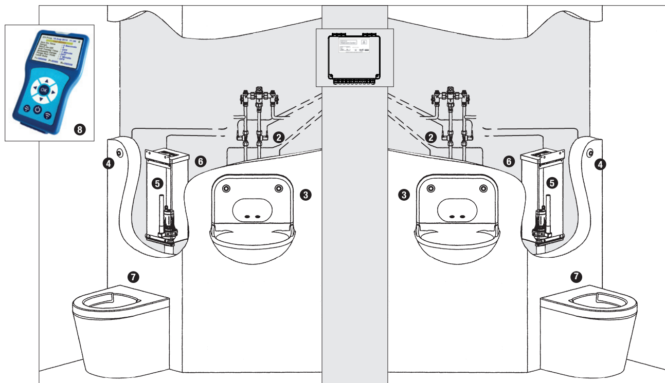
Fig. 3 Dual-Room WC and Basin
